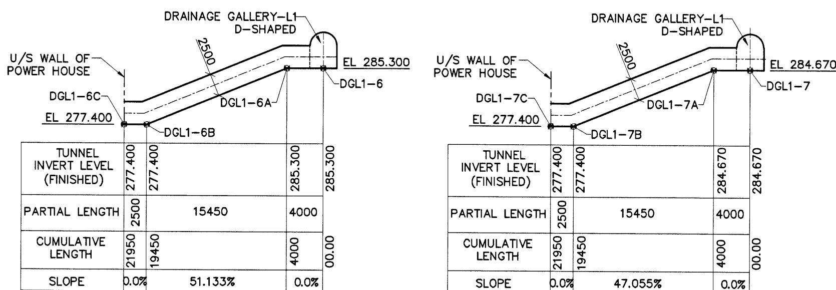
SECTION B (NTS)
